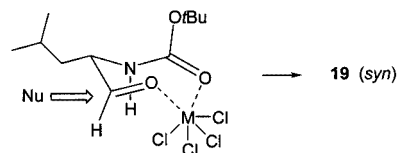
Figure 3. Stereochemical model for allylmethyl addition
