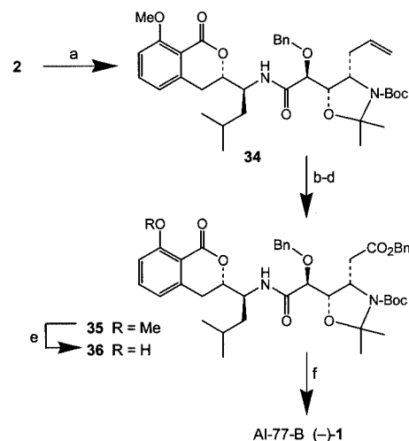
Scheme 6. (a) TFA, CH 2 Cl 2 , 0 °C, 30 min, then 3 , EDCI, DMAP, CH 2 Cl 2 , room temp., 12 h (72%); (b) O 3 , CH 2 Cl 2 , –78 to 23 °C, PPh 3 (98%); (c) NaClO 2 , 2-methyl-2-butene, NaH 2 PO 4 ·H 2 O, t BuOH/H 2 O (5:1) (99%); (d) Cs 2 CO 3 , MeOH/H 2 O (5:1), 30 min, then BnBr, DMF, 0 °C, 6 h (90%); (e) MgI 2 , THF, reflux, 5 min (93%); (f) H 2 , 10% Pd/C, Dowex® 50-X8, THF/MeOH (1:1), 23 °C, 12 h (75%)
