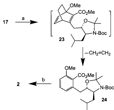
Scheme 3. (a) 1-Methoxy-1,3-cyclobutadiene, toluene, 175\text{ }^{\circ}\text{C} , 3 d (76%); (b) TsOH, \text{CH}_2\text{Cl}_2 , \text{H}_2\text{O} , 23\text{ }^{\circ}\text{C} , 20 min (97%)
