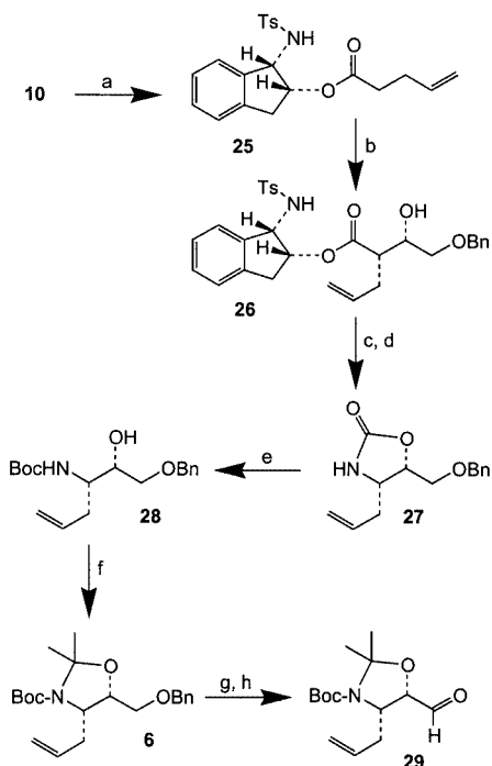
Scheme 4. (a) 4-Pentenoic acid, EDCI, DMAP, \text{CH}_2\text{Cl}_2 , 23\text{ }^{\circ}\text{C} , 4 h (99%); (b) \text{TiCl}_4 , i\text{Pr}_2\text{NEt} , 0\text{ to }23\text{ }^{\circ}\text{C} , 1 h, then \text{BnOCH}_2\text{CHO} , -78\text{ }^{\circ}\text{C} , 20 min (97%); (c) \text{LiOH} , \text{H}_2\text{O}_2 , \text{THF}/\text{H}_2\text{O} (3:1), 23\text{ }^{\circ}\text{C} , 12 h (96%); (d) DPPA, \text{Et}_3\text{N} , \text{CH}_2\text{Cl}_2 , reflux, 12 h (92%); (e) \text{Boc}_2\text{O} , \text{Et}_3\text{N} , DMAP, THF, 23\text{ }^{\circ}\text{C} , 2 h, then aqueous \text{NaOH}/\text{EtOH} (1:1) (96%); (f) DMP, p -TsOH, \text{CH}_2\text{Cl}_2 , 23\text{ }^{\circ}\text{C} , 6 h (92%); (g) \text{Li}/\text{NH}_3 , THF, -78\text{ }^{\circ}\text{C} , 5 min (95%); (h) (\text{COCl})_2 , DMSO, \text{Et}_3\text{N} , \text{CH}_2\text{Cl}_2 , -78\text{ to }0\text{ }^{\circ}\text{C} (95%)
