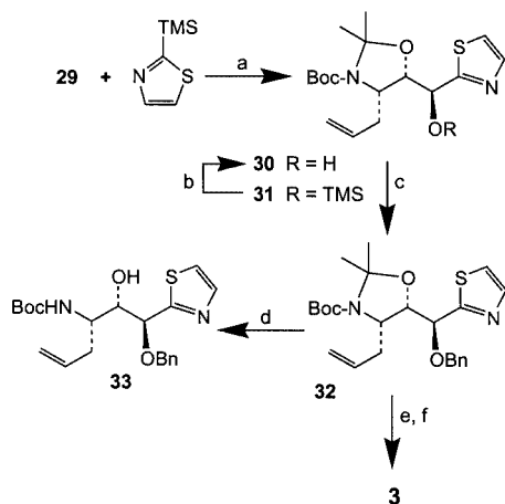
Scheme 5. (a) 2-TST, CH 2 Cl 2 , 23 °C, 6 h; (b) TBAF, THF, room temp., 20 min (85%, 29 to 30 ); (c) NaH, BnBr, n Bu 4 NI, THF, 12 h (95%); (d) p -TsOH·H 2 O, MeOH, 23 °C, 24 h (95%); (e) i. MeOTf, 4 Å molecular sieves, MeCN, 23 °C, 30 min; ii. NaBH 4 , MeOH, 0 °C, 30 min; iii. CuO, CuCl 2 ·H 2 O, MeCN/H 2 O (10:1), 23 °C, 10 min (82%); (f) NaClO 2 , NaH 2 PO 4 ·H 2 O, 2-methyl-2-butene, t BuOH/H 2 O (5:1) (98%)
