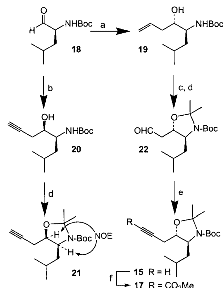
Scheme 2. (a) \text{SnCl}_4 , allyltributyltin, –78 °C, 1 h (94%, 92% de ); (b) \text{HC}\equiv\text{CCH}_2\text{Br} , Zn, DMF/ \text{Et}_2\text{O} (1:1), 0 to 23 °C, 12 h (67%, 84% de ); (c) DMP, TsOH, DCM, 23 °C, 1 h (99%); (d) \text{O}_3 , \text{PPh}_3 , DCM, –78 °C (97%); (e) \text{CH}_3\text{COC}(\text{N}_2)\text{PO}(\text{OMe})_2 , \text{Cs}_2\text{CO}_3 , i PrOH, 0 °C, 1 h, 23 °C, 11 h (97%); (f) n BuLi, \text{ClCO}_2\text{Me} , THF, –78 °C, 10 min (99%)
