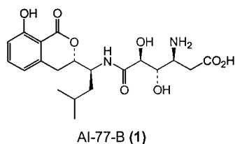
Figure 1. Structure of AI-77-B
