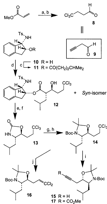
Scheme 1. (a) NaOH, BnEt 3 NCl, CHCl 3 , H 2 O, 0 °C, 2 h (32%); (b) DIBAL, CH 2 Cl 2 , –78 °C, 1.5 h (95%); (c) 4-methylvaleric acid, EDCI, DMAP, 23 °C, 2 h (99%); (d) TiCl 4 , i Pr 2 NEt, 0 to 23 °C, 1 h, then 8 , –78 °C, 10 min (90%, 90% de ); (e) LiOH, H 2 O 2 , THF, H 2 O, room temp., 12 h (97%); (f) DPPA, Et 3 N, CH 2 Cl 2 , reflux, 12 h, (94%); (g) Boc 2 O, DMAP, Et 3 N, THF, room temp., 3 h, then NaOH, EtOH, H 2 O, room temp., 5 min (91%); (h) DMP, TsOH, CH 2 Cl 2 , 23 °C, 15 min (97%); (i) n BuLi, TMEDA, THF, –78 °C, 20 min, then ClCO 2 Me (85%); (j) n BuLi, THF, –78 °C, 10 min (88%)
