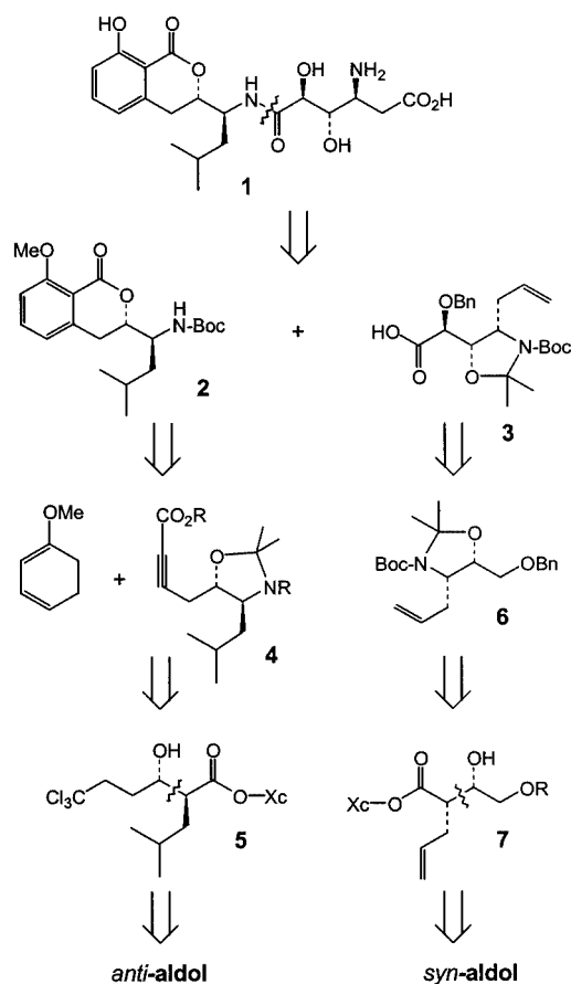
Figure 2. Retrosynthesis of AI-77-B
